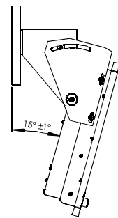
Wall mounted
